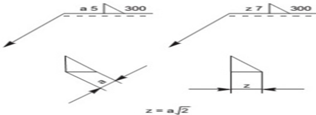
Fig. 11.9. Dimensioning of welds
