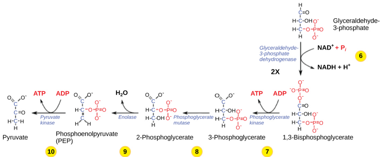
Figure 9.1.2: The second half of glycolysis involves phosphorylation without ATP investment (step 6) and produces two \text{NADH} and four \text{ATP} molecules per glucose.
