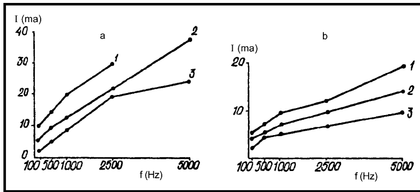
Figure 5. Maximum tolerable current (1), current required to achieve 60% of the maximum electrically induced torque (2) and motor thresholds (3) measured at different alternating current frequencies in the range 100 Hz to 5 kHz using continuous alternating current. I=intensity, f=frequency. Reproduced from Andrianova et al. 12
