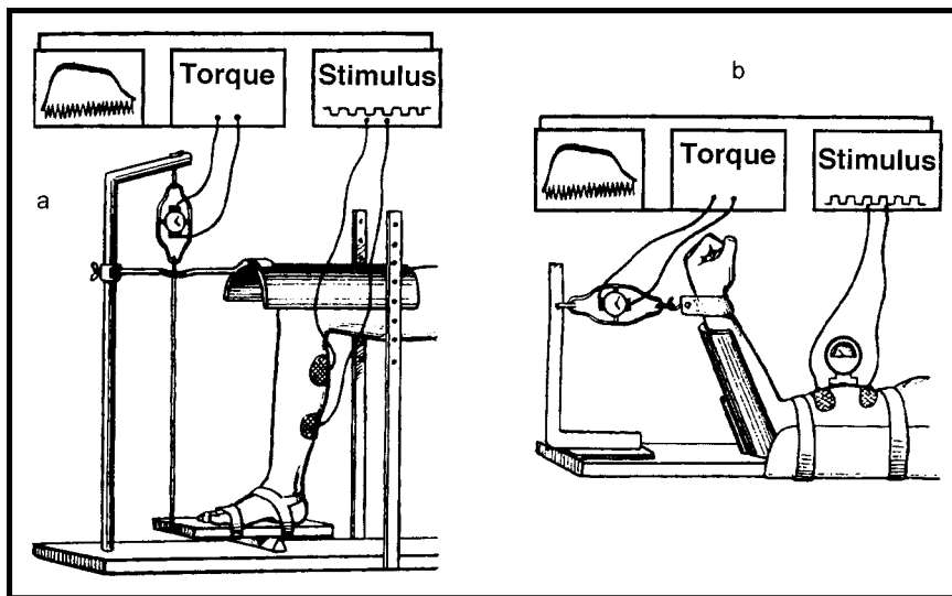
Figure 1. Apparatus used for measurement of maximum voluntary contraction and maximum electronically induced torque of (a) triceps surae muscles and (b) biceps brachii muscles. A skin-surface-mounted device was used to measure the hardness of the biceps brachii muscles. Reproduced from Kots and Xvilon. 11
