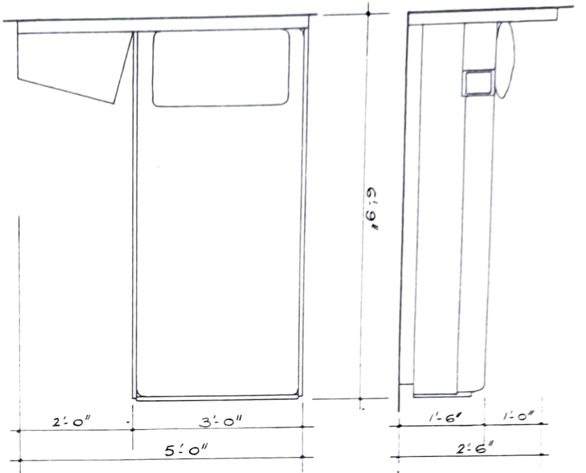
PLAN AND ELEVATIONS OF A SINGLE BED scale : 1" = 2'-0"
