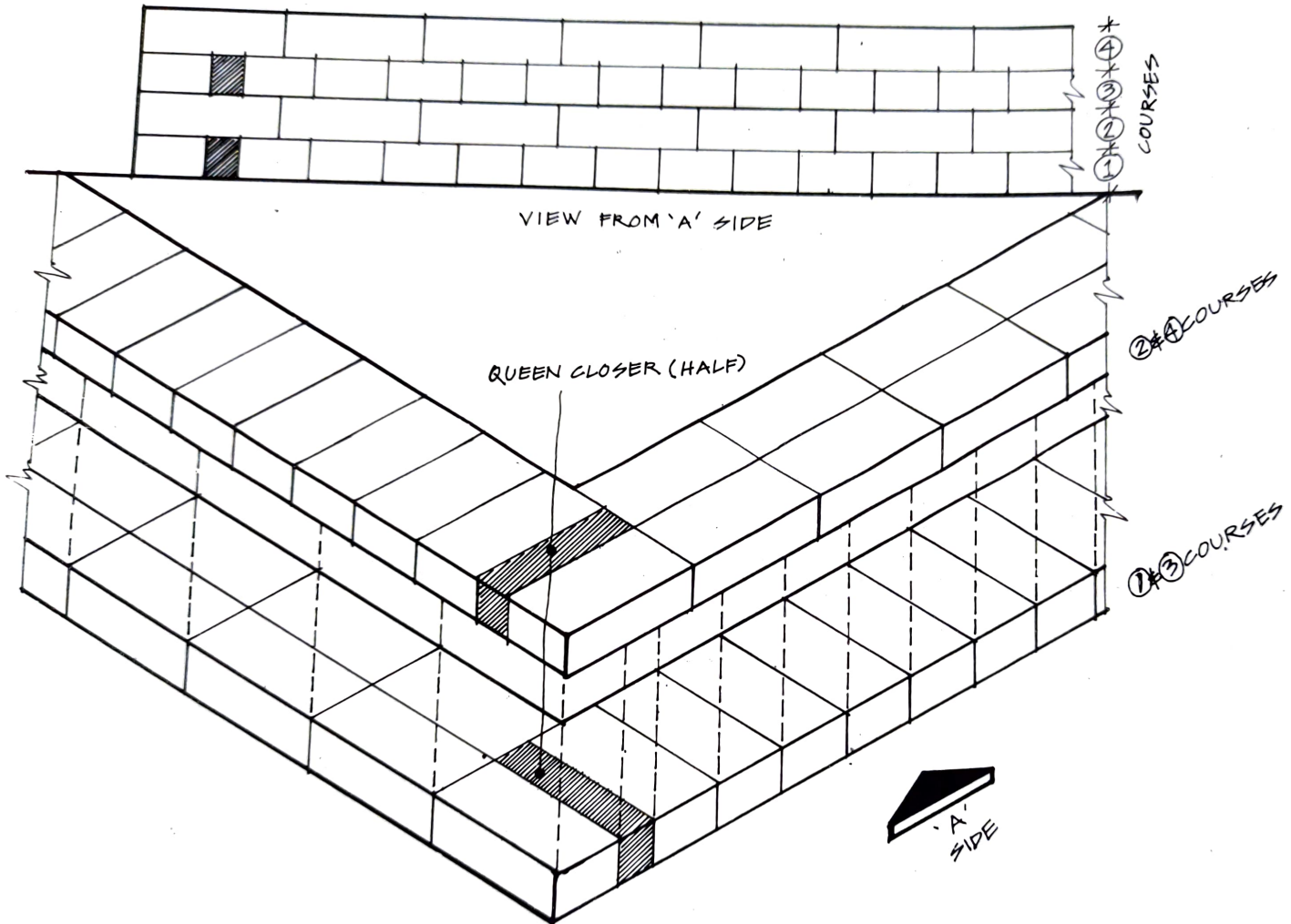
ENGLISH BOND OF ONE BRICK WALL (SCALE: 1:10 or 10CM = 1METER)
