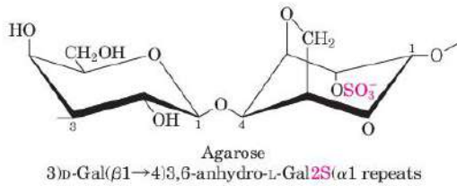
FIGURE 7-23 The structure of agarose. The repeating unit consists of D-galactose (β1→4)-linked to 3,6-anhydro-1-galactose (in which an ether ring connects C-3 and C-6). These units are joined by (α1→3) glycosidic links to form a polymer 600 to 700 residues long. A small fraction of the 3,6-anhydrogalactose residues have a sulfate ester at C-2 (as shown here).
