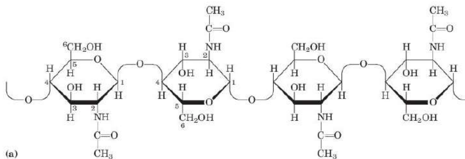
FIGURE 7-18 Chitin. (a) A short segment of chitin, a homopolymer of N -acetyl- \beta -glucosamine units in ( \beta 1 \rightarrow 4 ) linkage. (b) A spotted June beetle ( Pellidnota punetata ), showing its surface armor (exoskeleton) of chitin.
