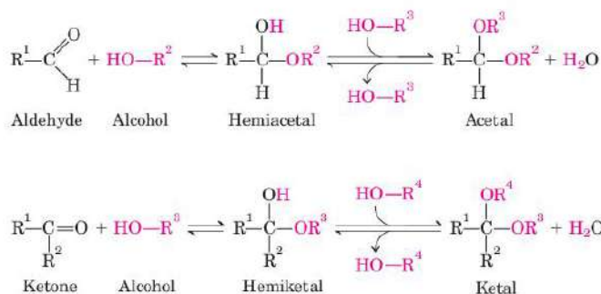
FIGURE 7-5 Formation of hemiacetals and hemiketals.
