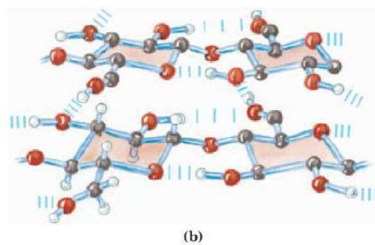
FIGURE 7-16 The structure of cellulose. (a) Two units of a cellulose chain; the D-glucose residues are in (\beta 1 \rightarrow 4) linkage. The rigid chair structures can rotate relative to one another. (b) Scale drawing of segments of two parallel cellulose chains, showing the conformation of the D-glucose residues and the hydrogen-bond cross-links. In the hexose unit at the lower left, all hydrogen atoms are shown; in the other three hexose units, the hydrogens attached to carbon have been omitted for clarity as they do not participate in hydrogen bonding.
