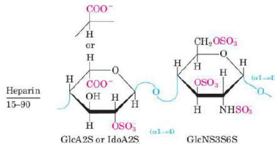
FIGURE 7-24 Repeating units of some common glycosaminoglycans of extracellular matrix. The molecules are copolymers of alternating uronic acid and amino sugar residues, with sulfate esters in any of several positions. The ionized carboxylate and sulfate groups (red) give these polymers their characteristic high negative charge. Heparin contains primarily iduronic acid (IdoA) and a smaller proportion of glucuronic acid (GlcA), and is generally highly sulfated and heterogeneous in length. Heparan sulfate (not shown) is similar to heparin but has a higher proportion of GlcA and fewer sulfate groups, arranged in a less regular pattern.
