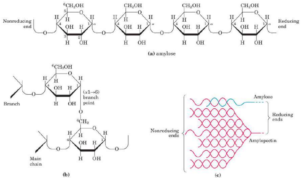
FIGURE 7-15 Amylose and amylopectin, the polysaccharides of starch. (a) A short segment of amylose, a linear polymer of D-glucose residues in (\alpha 1 \rightarrow 4) linkage. A single chain can contain several thousand glucose residues. Amylopectin has stretches of similarly linked residues between branch points. (b) An (\alpha 1 \rightarrow 6) branch point of amylopectin. (c) A cluster of amylose and amylopectin like that believed
