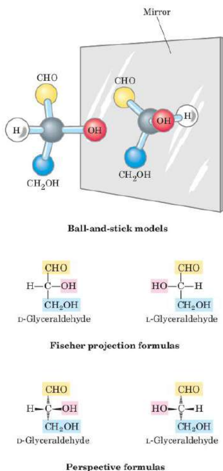
FIGURE 7-2 Three ways to represent the two stereoisomers of glyceraldehyde. The stereoisomers are mirror images of each other. Ball-and-stick models show the actual configuration of molecules. By convention, in Fischer projection formulas, horizontal bonds project out of the plane of the paper, toward the reader; vertical bonds project behind the plane of the paper, away from the reader. Recall (see Fig. 1-17) that in perspective formulas, solid wedge-shaped bonds point toward the reader, dashed wedges point away.
