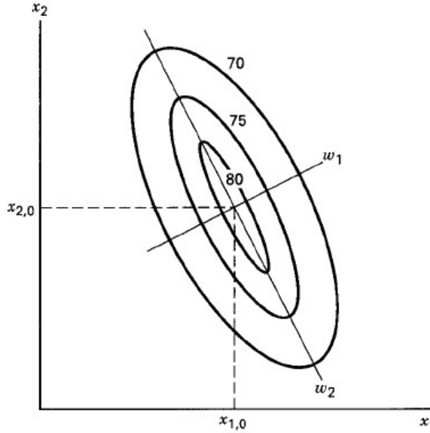
Canonical form of the second order model
